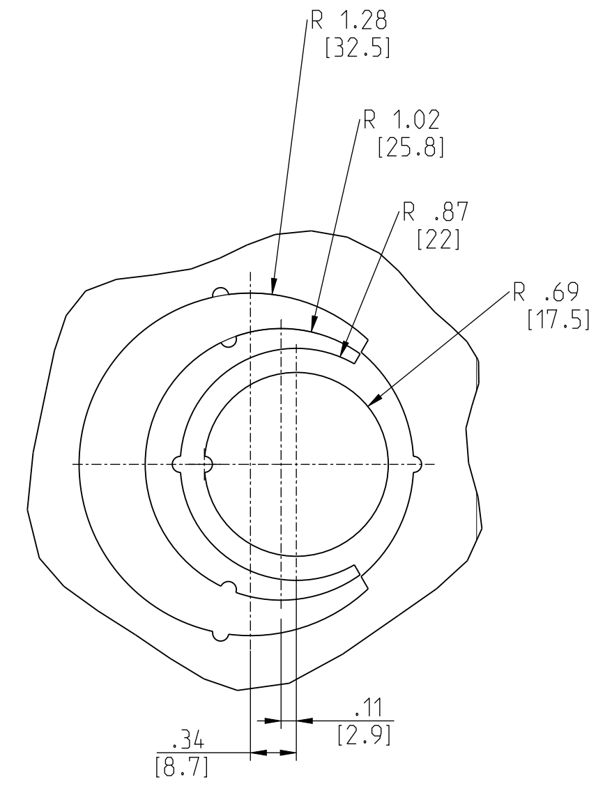
DETAIL B
