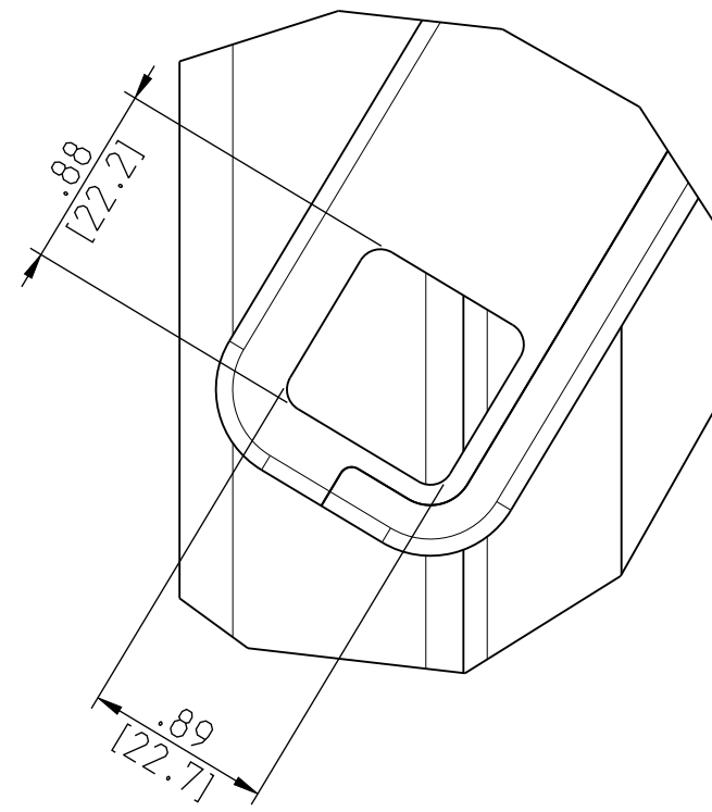
DETAIL A
