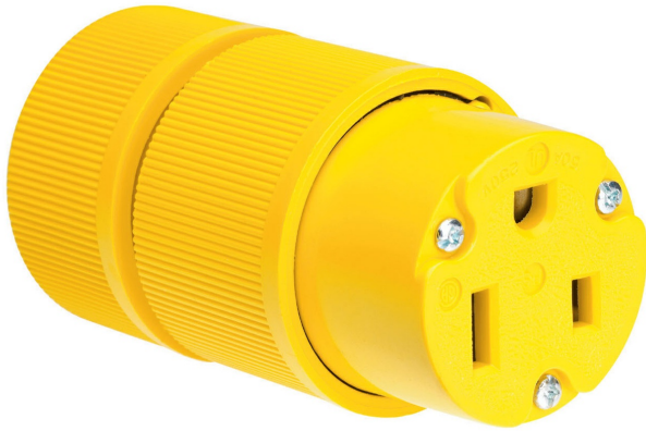
Gator GripConnector, 2-Pole 3-Wire 50A 250V Grounding, Yellow
