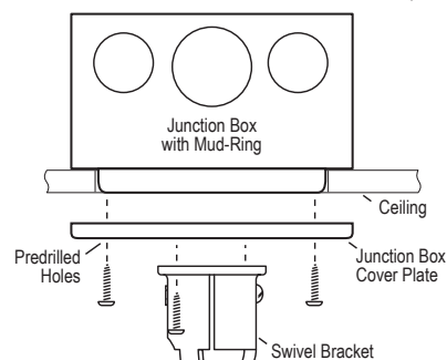
Junction Box Cover Plate Installation Wattstopper recommends using a 3.0" mudring with a 4" octagonal box.
