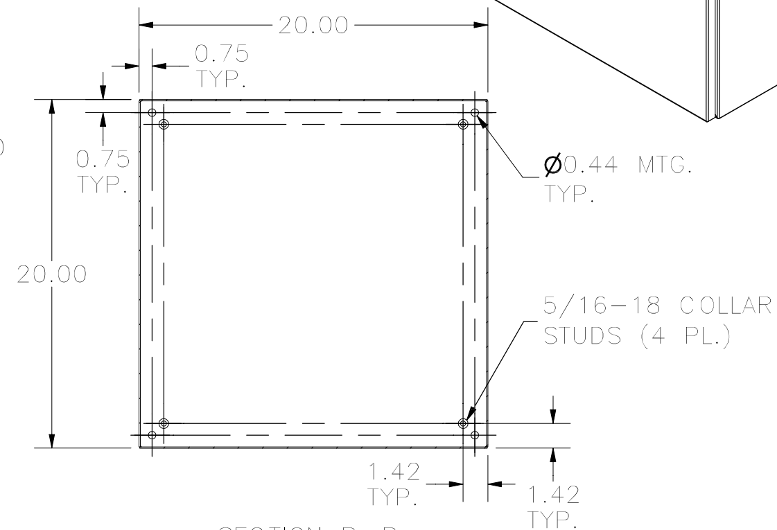
SECTION B-B (INSIDE BACK OF ENCLOSURE)
