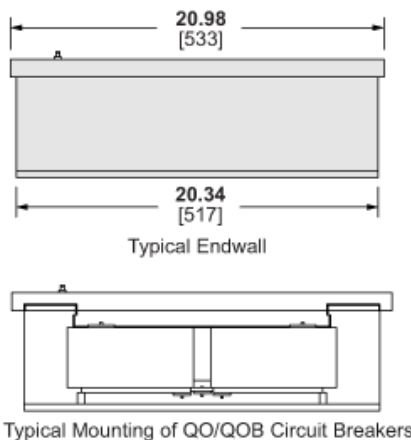
Typical Mounting of QO/QOB Circuit Breakers
