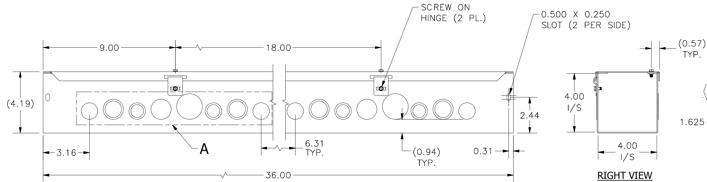
FRONT VIEW
