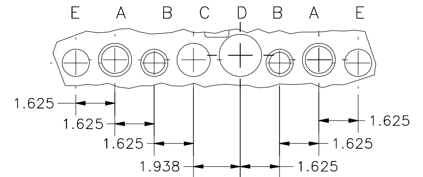
DETAIL A (2 PL. PER SIDE) K.O. PATTERN DESCRIPTION
