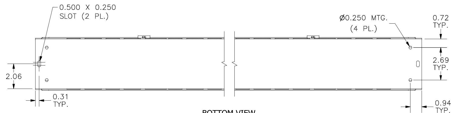
BOTTOM VIEW
