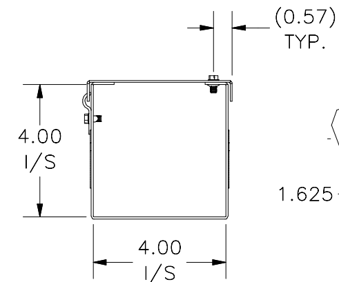
RIGHT VIEW
