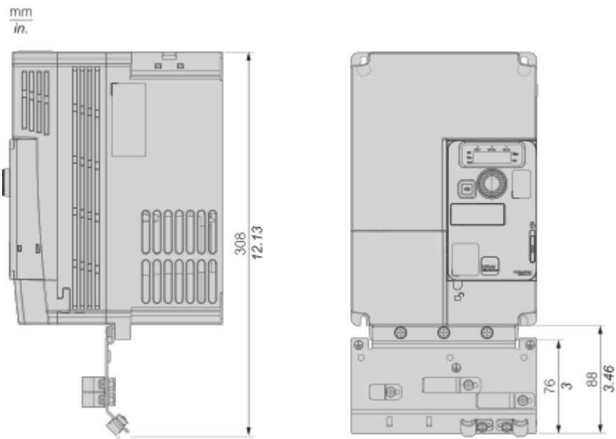
Right and Front View with EMC Plate
