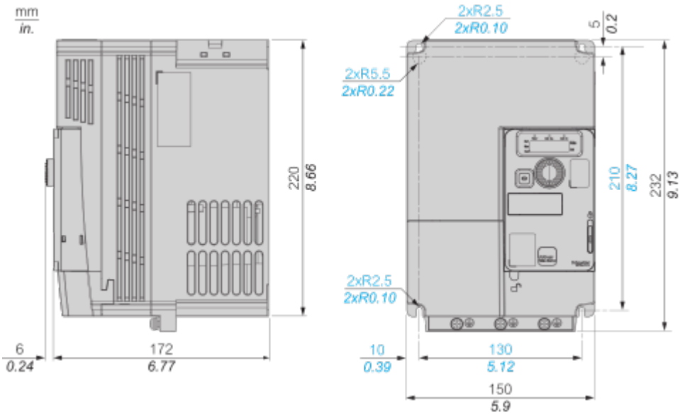
Right and Front View with EMC Plate
