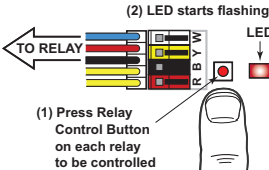
Step 2. RELAY DRIVER CARD
