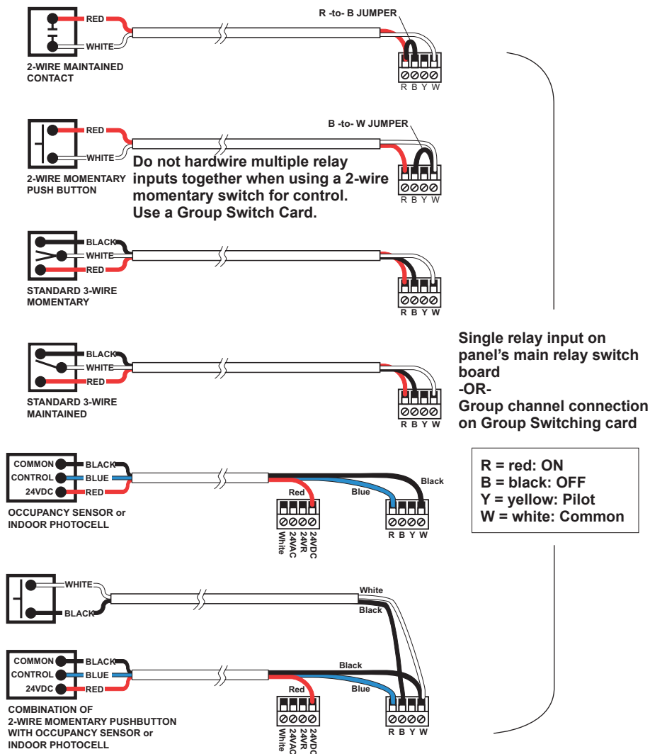
Figure 9: Low voltage switch and sensor wiring.
