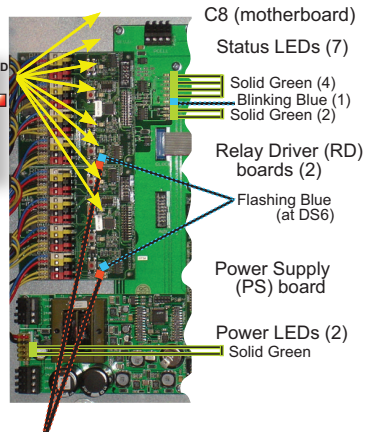
Figure 8: Relay Control Buttons & Status LEDs
