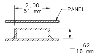
SECTION Z-Z 87784698
