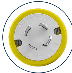
Corrosion resistant blades, contacts and assembly screws
