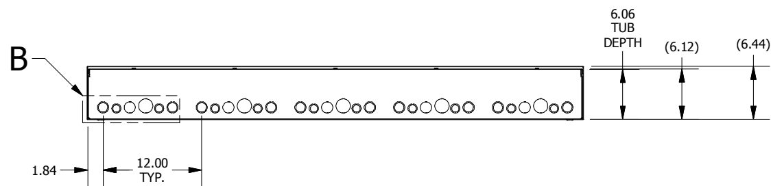
BOTTOM VIEW
