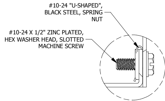
DETAIL A (5 PL.) (LID ATTACHMENT DETAIL)
