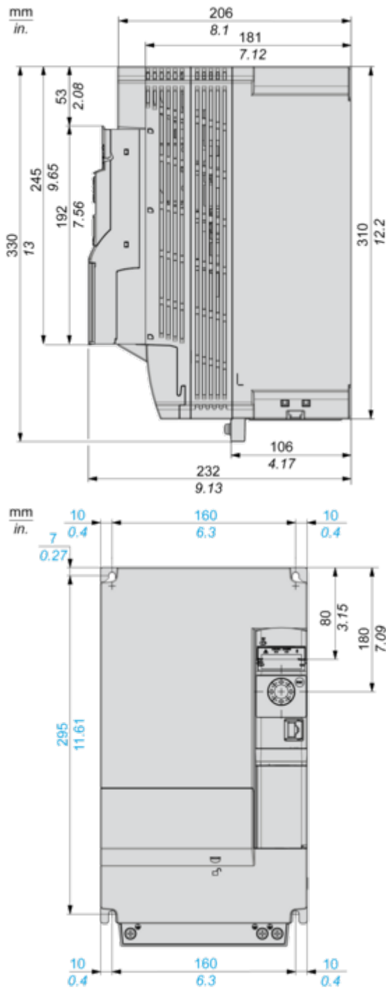
Right and Front View with EMC Plate
