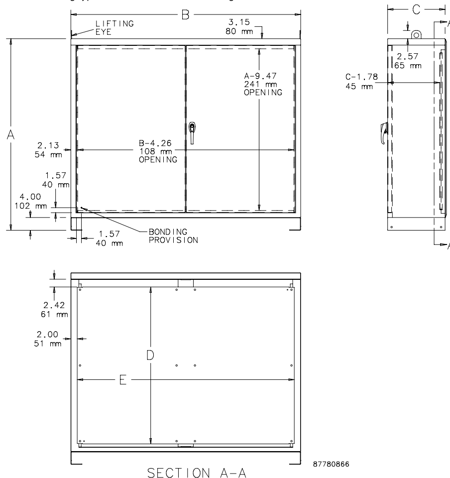
Free-Standing Type 1 Two-Door Enclosures Drawing
