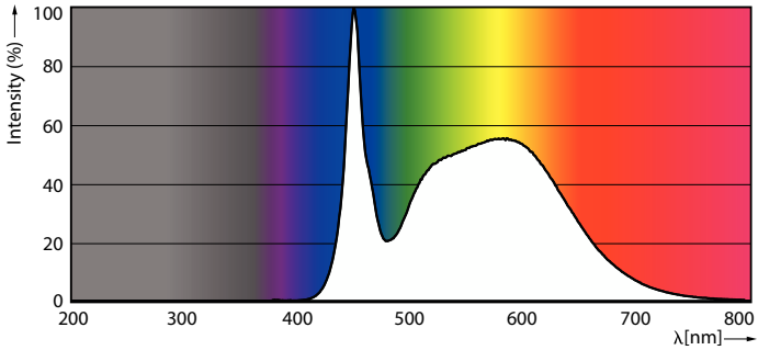
Spectral Power Distribution Colour - 150CC/LED/850/LS EX39 G2 BB 277-480V 3/1
