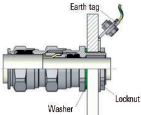
WITH WASHER: IP66 / IP68
