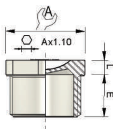
Ordering codes - Hex head stopping plug
