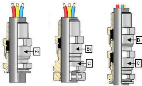
ADE-1F2 A (Anchorage)
