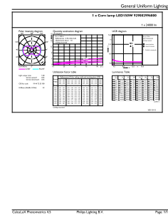
General uniform lighting - 150CC/LED/850/LS EX39 G2 BB 3/1
