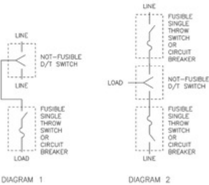
DIAGRAM 1 AND 2 ILLUSTRATE METHODS OF APPLYING FUSES TO DOUBLE THROW SWITCHES WHEN REQUIRED.
