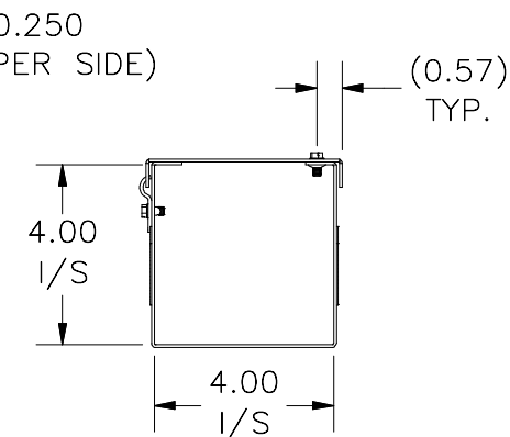
RIGHT VIEW
