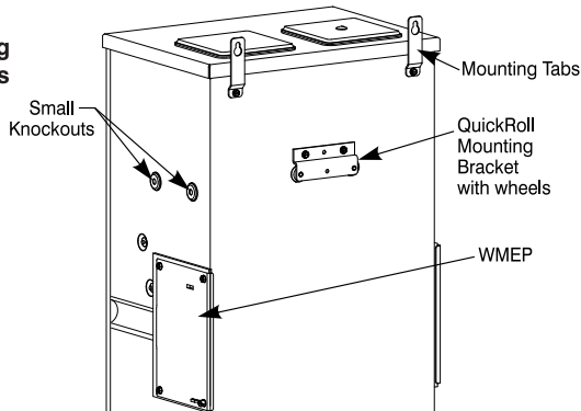
Fig. 2: Detail for Installing Mounting Brackets
