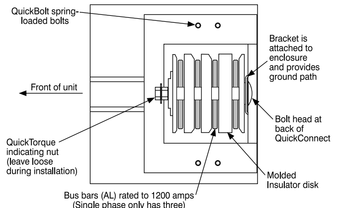
Fig. 6: QuickConnect Detail
