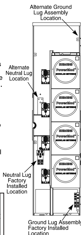
Fig. 11: Position of Ground and Neutral Lugs
