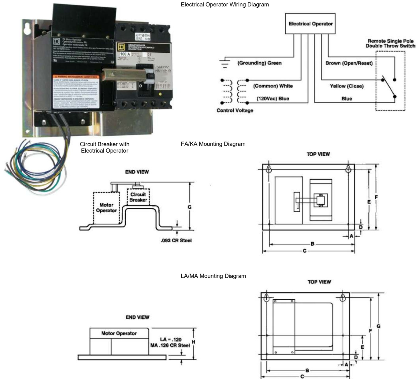
Figure 23: Electrical Operator Side Mount Dimensions and Wiring Diagram
