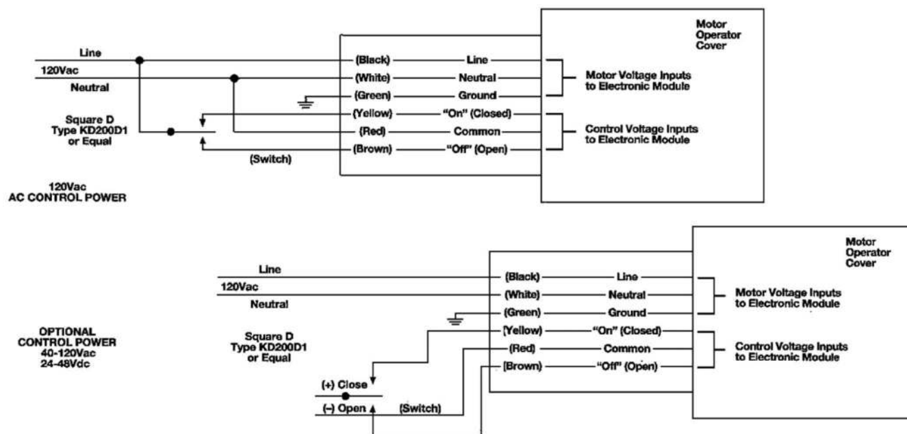
Figure 25: PAMO2 Electrical Operator Suggested Wiring Diagrams
