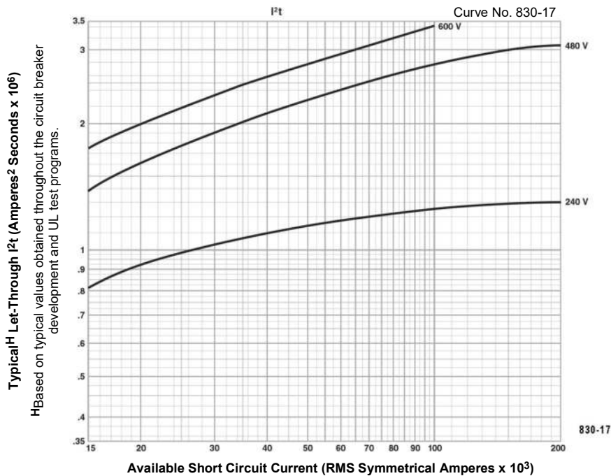
I-LIMITER CURRENT LIMITING CIRCUIT BREAKERS LI Series 2, 3 and LXI Series 2B, 3B 600 A Frame at 240, 480 and 600 Vac, 3Ø 450–600 A Curve No. 830-17 Let-Through I^2t and 830-18 Peak Let-Through Current I_p
