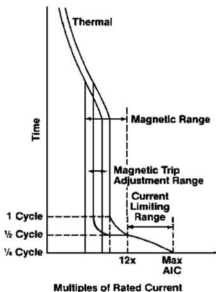
Figure 4: FI Characteristic Tripping Curve
