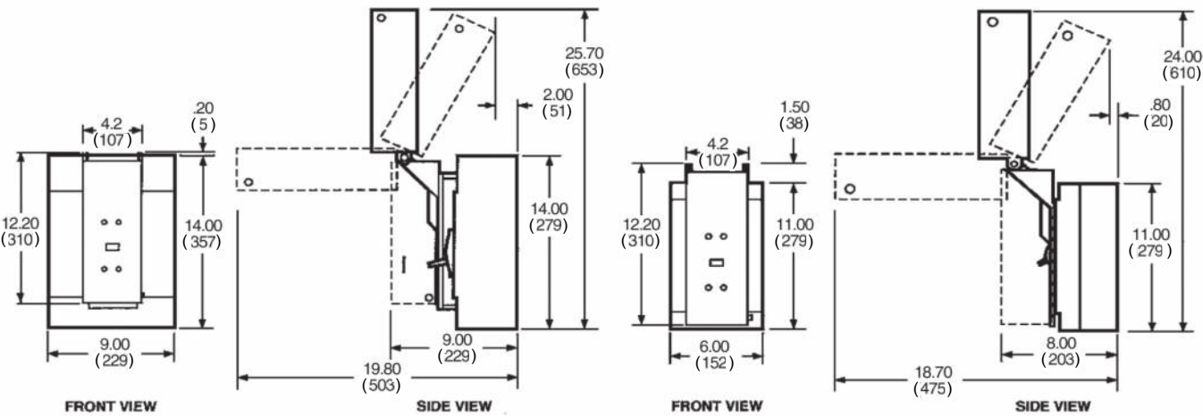
Figure 24: Top Mount Electrical Operator Dimensions and Wiring Diagrams
