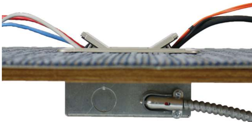
CAF3 installed in wood floor with Walkerflex® Wiring System.
