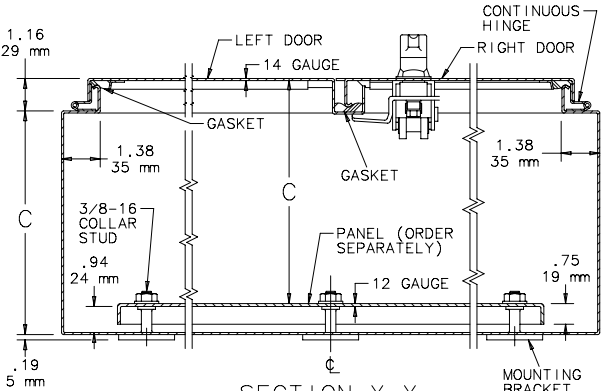
SECTION X-X
