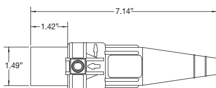
Male Connector
