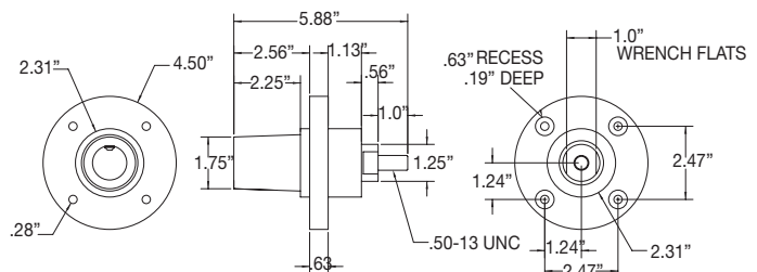
Female Receptacle 90° angle
