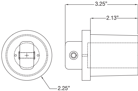
Male Cap
