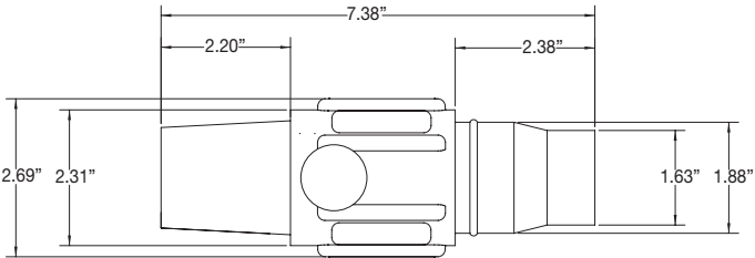
Female Connector
