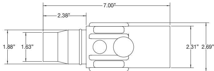
Male Connector
