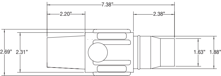
Female Connector
