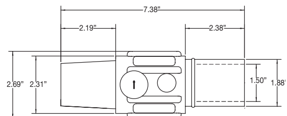
Female Connector
