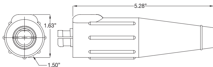
Male Plug
