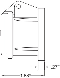
Snap Back Enclosure Assembly
