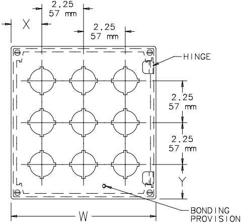
VIEW X-X
