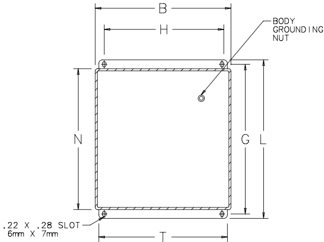
SECTION Y-Y
