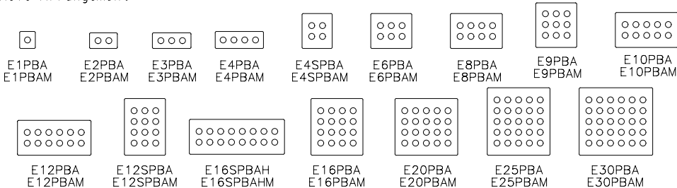
Hole Arrangement
