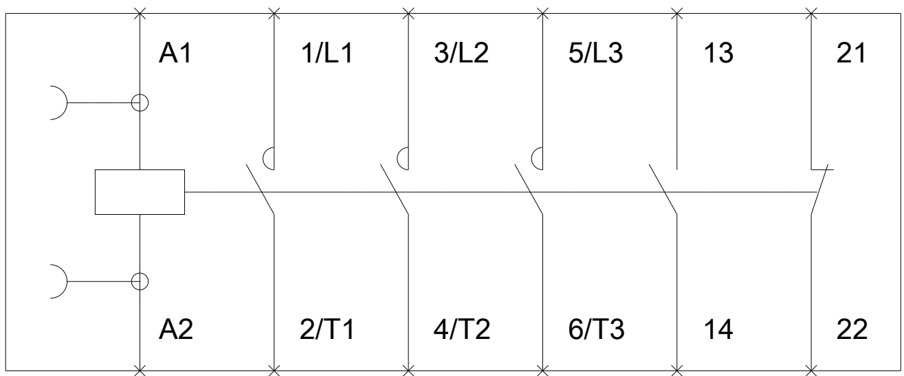
LEN00C003 Wiring Diagram
