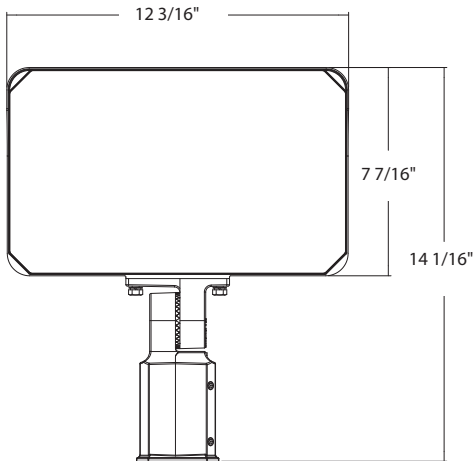
Slipfitter Mount
