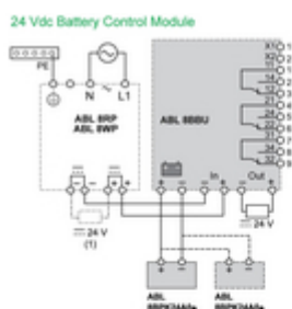
24 Vdc Battery Control Module
