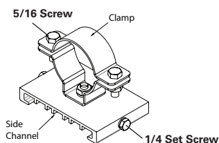
Figure 7. PM KIT – Pole Mount Details
