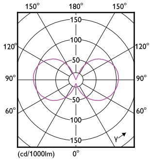
Light Distribution Diagram - 25GC/LED/850/ND E26 BB 6/1
