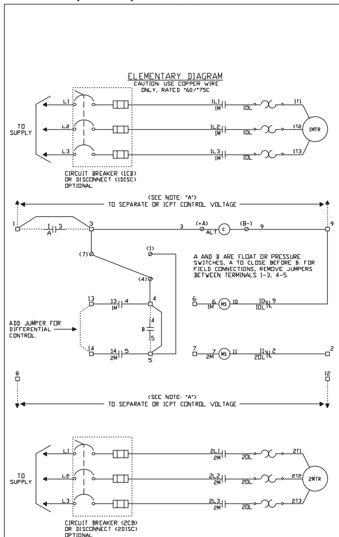
Standard Duplex Pump Panel (92)
