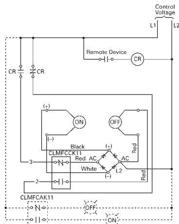
Connection for 2-Wire Control CLMOC , CLMOD , CLMOE , and CLMOF
