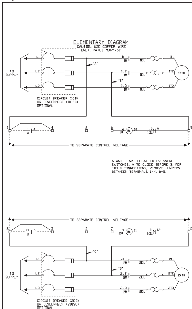
Duplex Panel w/o alternator (95)
