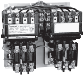
2S2W starter (Amb. Comp. Bimetal OL)
