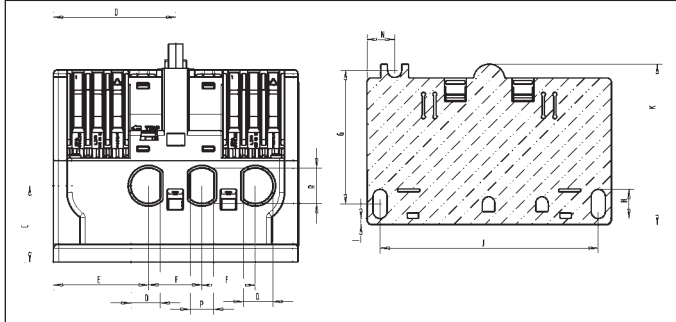
Dimensions "B" Frame—ESP200 Solid State Overload
