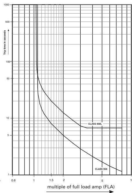
Time - Current - Characteristics CLASS 958, 958L
