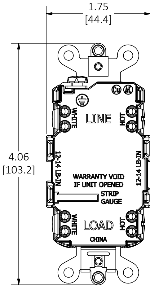
BACK VIEW (SAME FOR ALL DEVICES)
