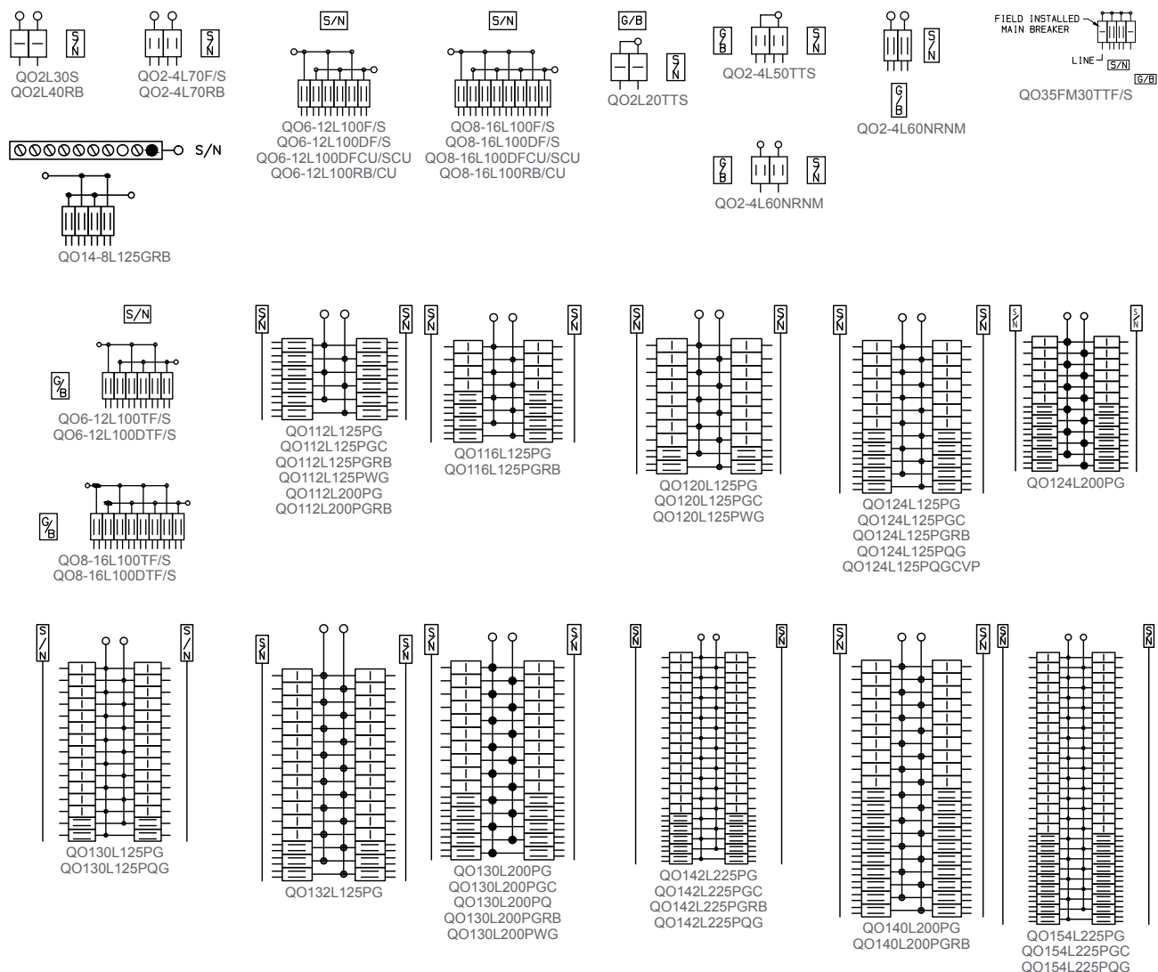
Figure 3 - QO Load Centers 1Ø – Main Lugs
