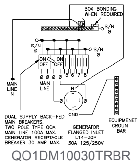
Figure 5 - Backup Power Solutions
