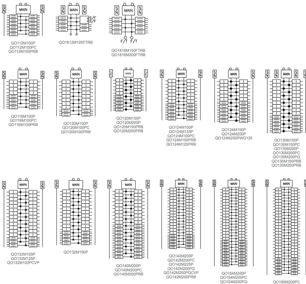
Figure 4 - QO Load Centers 1Ø – Main Circuit Breaker
