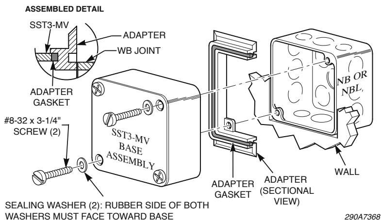
Figure 2 Mounting with an NB or NBL box
