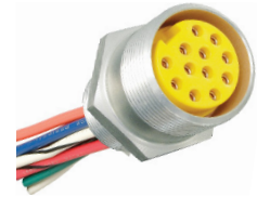
MR9F4BC100A Style III Female Receptacle
