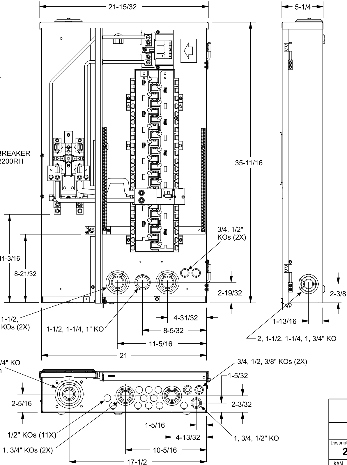
View Shown Without Covers, Door, Deadfront
