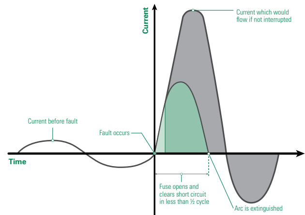
Figure 13 – Current-limiting Fuse
