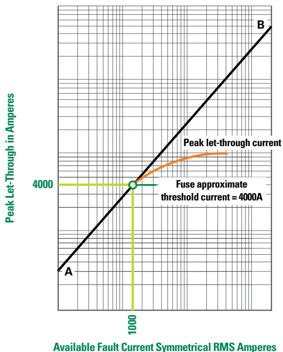
Figure 19 – Determining Threshold Current from Peak Let-through Chart
