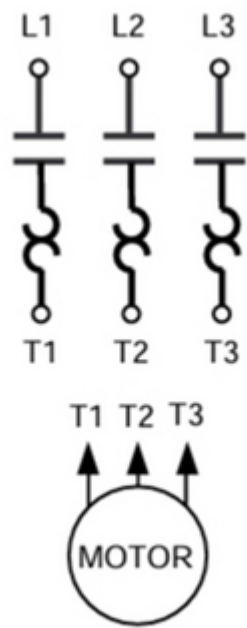
3-Pole, 3-Phase
