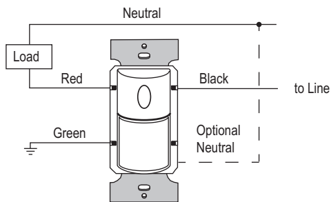
Single-level wiring
