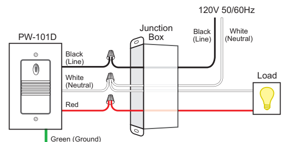
Wiring for PW-101D with a neutral connection.
