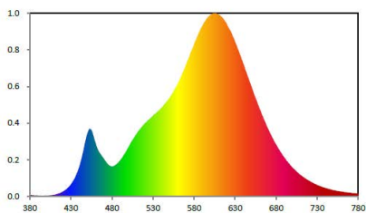
Spectral Power Distribution
