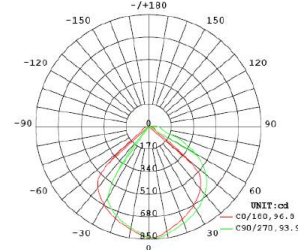
Luminous Intensity Distribution
