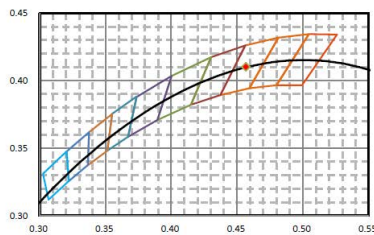
7-Step Chromaticity Quadrangles
