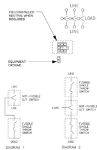
DTU366 DIAGRAM 1 AND 2 ILLUSTRATE METHODS OF APPLYING FUSES TO DOUBLE THROW SWITCHES WHEN REQUIRED.
