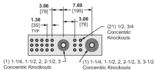
Endwall with Knockouts (Other Endwall is Blank)
