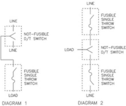
DIAGRAM 1 AND 2 ILLUSTRATE METHODS OF APPLYING FUSES TO DOUBLE THROW SWITCHES WHEN REQUIRED.
