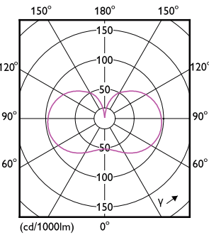
Light Distribution Diagram - 19GC/LED/850/ND E26 BB 6/1
