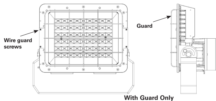
With Guard Only Figure 6
