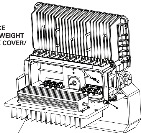
Cover/heat sink
