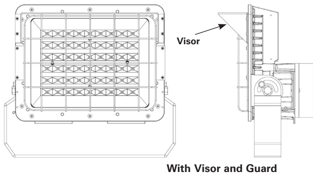
With Visor and Guard Figure 5
