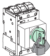
Padlocking Direct Rotary Handle
