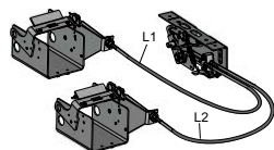
Dual-Cable Operating Mechanism
