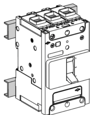
Mounting on rails (Two mounting screws)
