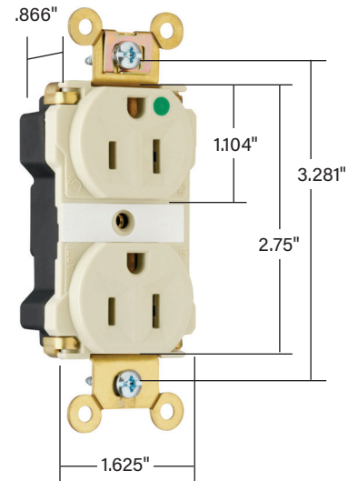
Dimensions for 15 & 20 Amp PT8200I
