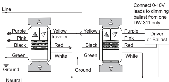
Typical Multi-Way Wiring (DW-311 or DW-311-347 up to 4 sensors)
