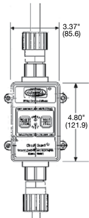
Dimensional Drawing
